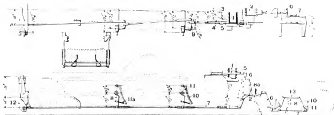
Figs. 2650-2652. General Arrangement of Foundation Brake Gear for Atlantic (4-4-2) Locomotive. Pennsylvania Railroad.
